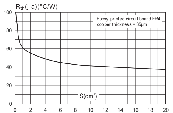
Fig.12 Thermal resistance junction to ambient versus copper surface under tab (DPAK)
