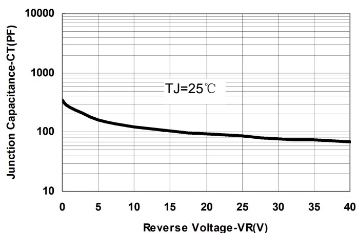
Fig.1-Typical Junction Capacitance
