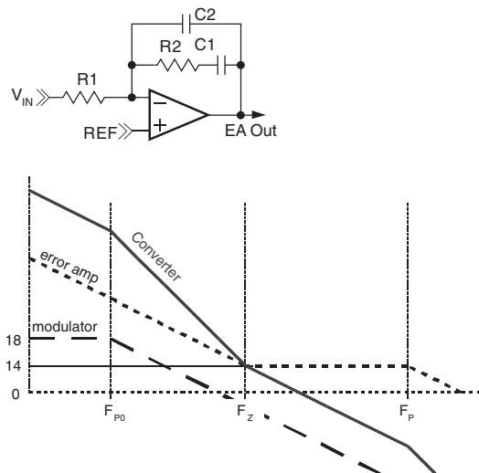
Figure 13. Compensation
