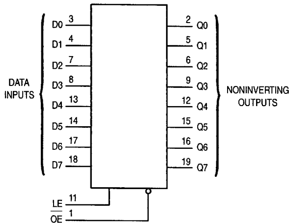
LOGIC DIAGRAM
