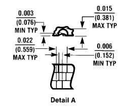
Ceramic Leadless Chip Carrier Package (E) Order Number 54LS20LMQB NS Package Number E20A
