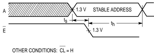
Figure 6. Setup Time, Address to Enable (See Notes 1 and 2)
