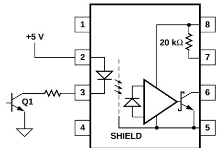
Figure 19. Not Recommended Open Collector LED Drive Circuit.
