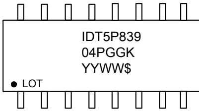
16-pin TSSOP
