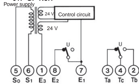
61F-GP-N8H
