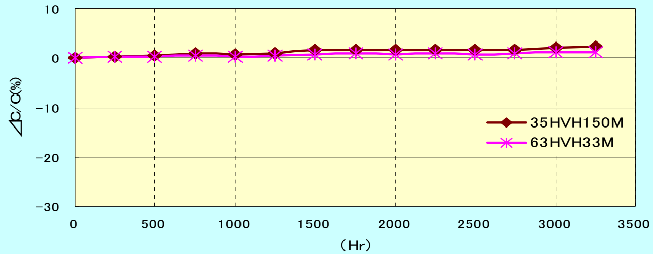
Capacitance change rate(120Hz)
