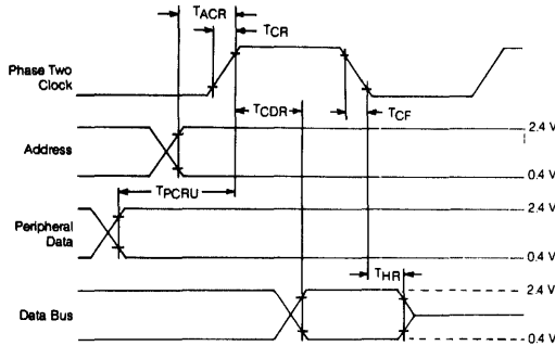
Figure 21. Read Timing Characteristics
