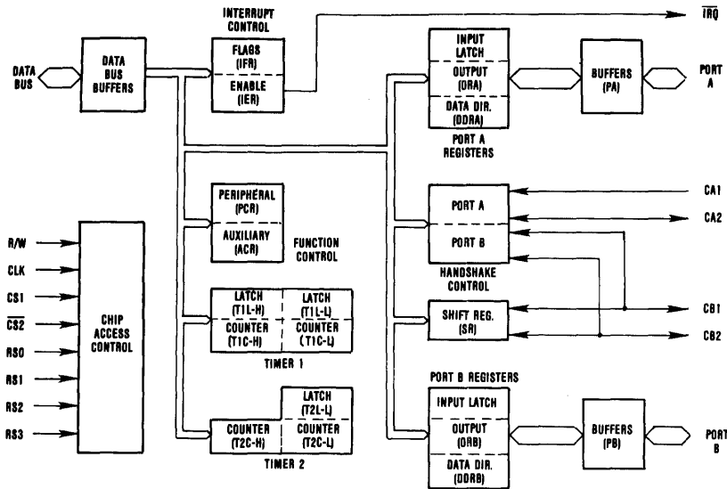
Figure 1. 6522 Block Diagram
