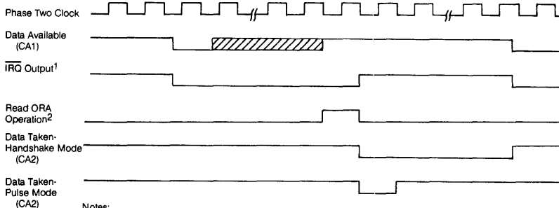
Figure 3. Read Handshake Timing Sequence
