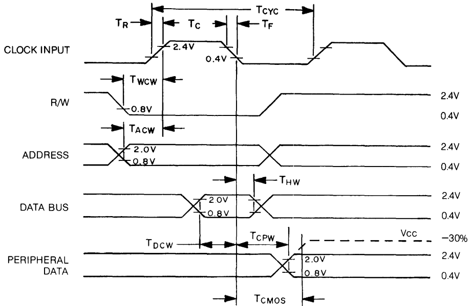
Figure 2 Write Timing Characteristics
