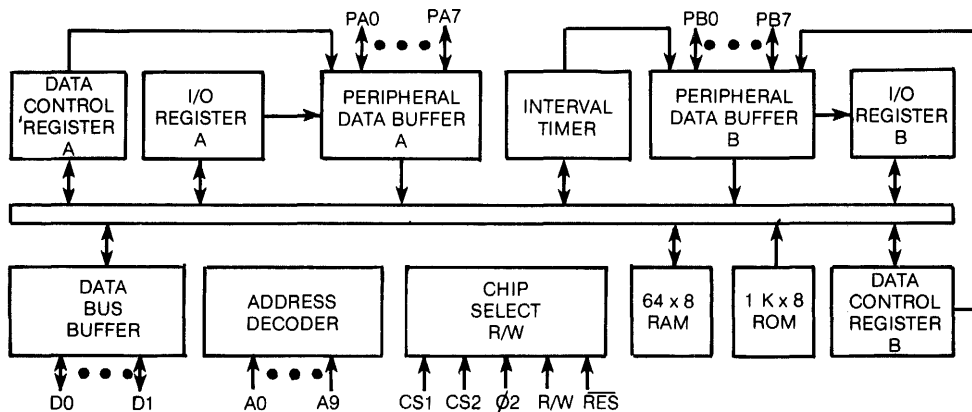
Figure 1. 6530 Block Diagram
