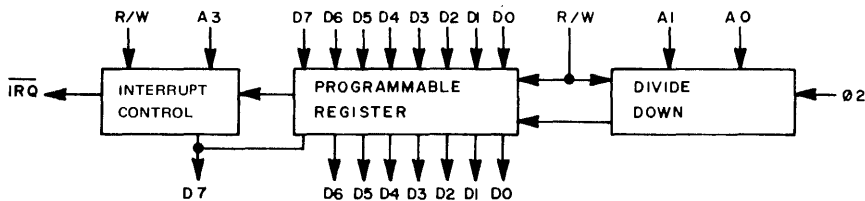
Figure 4. Basic Elements of Interval Timer
