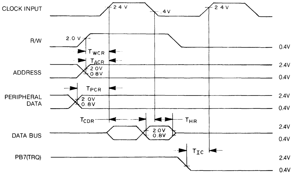
Figure 3 Read Timing Characteristics
