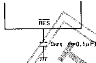
Fig. 4 Reset Circuit
