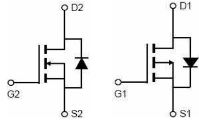
N-channel P-channel
