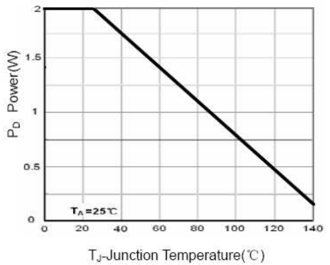
Figure 8 Power Dissipation
