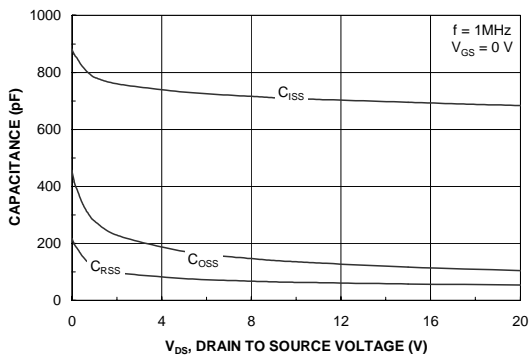
Figure 18. Capacitance Characteristics.
