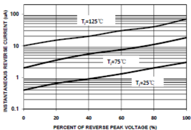
FIG 3-TYPICAL REVERSE CHARACTERISTICS
