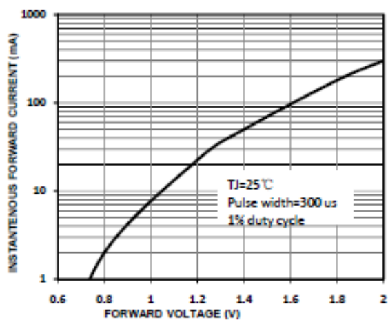
FIG 2-TYPICAL FORWARD CHARACTERISTICS
