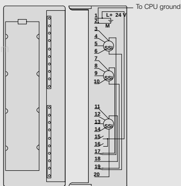
Fig. 1/13 Terminal connection diagram of the SM 338 POS input module
