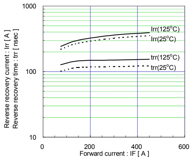
Reverse recovery characteristics (typ.) Vcc=600V, VGE=±15V, RG=2.0Ω
