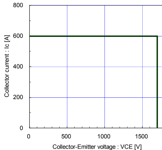
Reverse bias safe operating area (max.) +VGE=15V, -VGE ≤ 15V, Rg ≥ 1.5Ω, Tj ≤ 125°C Stray inductance ≤ 100nH
