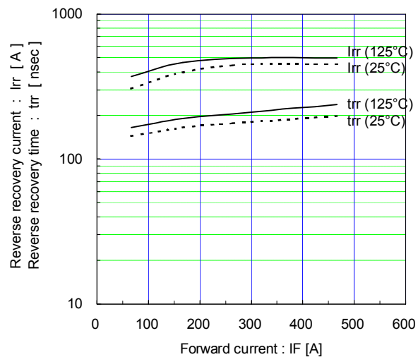
Reverse recovery characteristics (typ.) V_{cc}=900V , V_{GE}=\pm 15V , R_g=1.5\Omega
