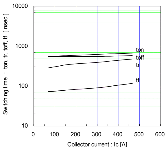
Switching time vs. Collector current (typ.) Vcc=900V, VGE=±15V, Rg=1.5Ω, Tj= 25°C
