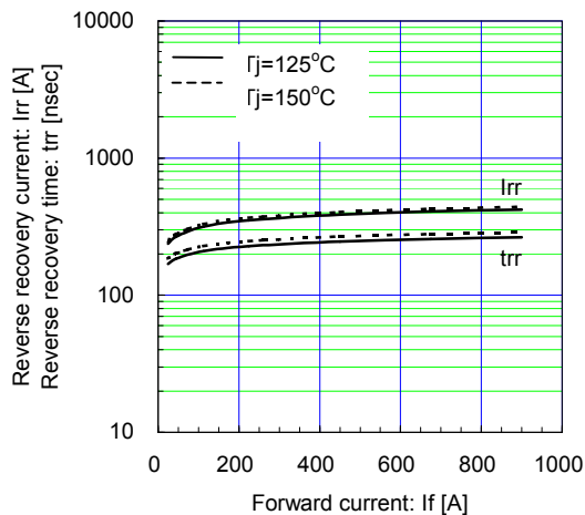
Reverse Recovery Characteristics (typ.) V_{cc}=600\text{V} , V_{ge}=\pm 15\text{V} , R_g=0.52\Omega , T_j=125^\circ\text{C} , 150^\circ\text{C}
