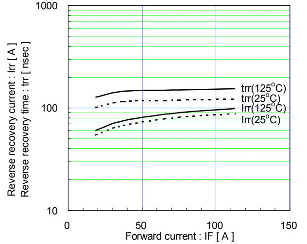
Reverse recovery characteristics (typ.) Vcc=600V, VGE=±15V, RG=9.1Ω
