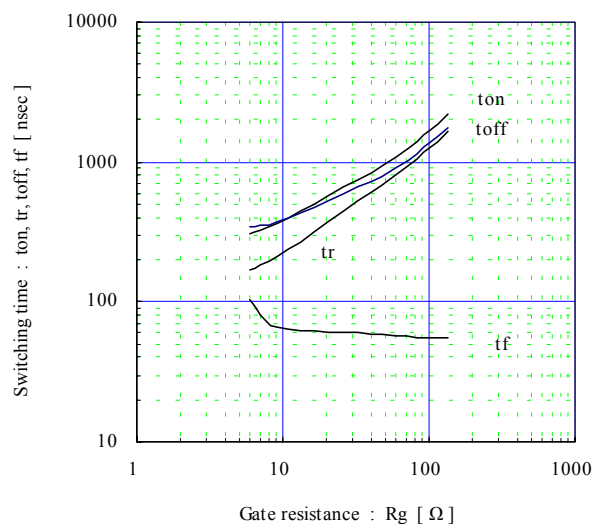
Switching time vs. Gate resistance (typ.) V_{cc}=600V, I_c=75A, V_{GE}=\pm 15V, T_j=25^\circ C
