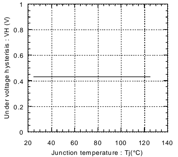
Under voltage hysteresis vs. Junction temperature
