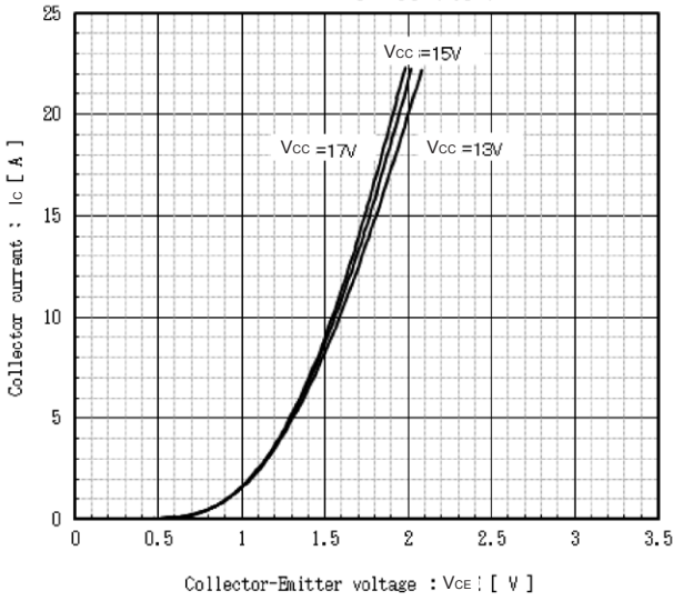
Collector current vs. Collector-Emittter voltage T_J = 25^\circ\text{C} [Chip] (typ.)
