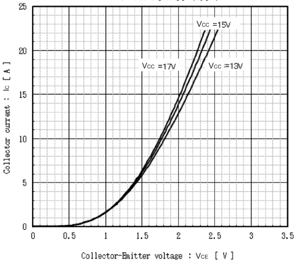
Collector current vs. Collector-Emittter voltage T_J = 125^\circ\text{C} [Chip] (typ.)
