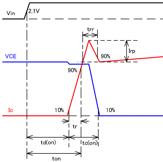
Fig.2-1: Switching waveforms
