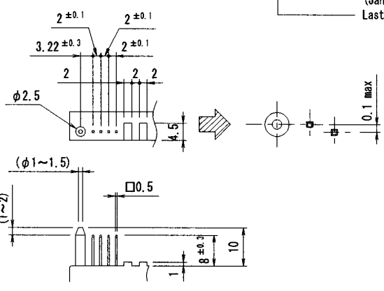
Details of control terminals Dimensions in mm
