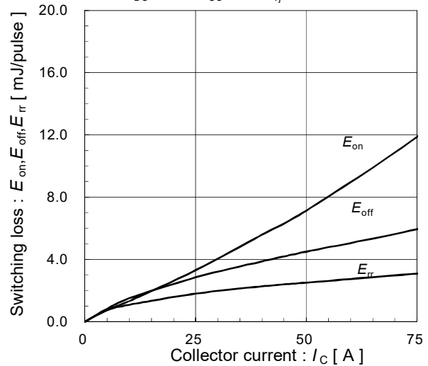
Switching loss vs. Collector current (typ.) V_{DC}=600\text{V}, V_{CC}=15\text{V}, T_{vj}=125^\circ\text{C}
