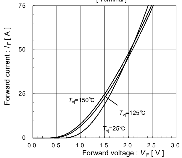
Forward current vs. Forward voltage (typ.) [ Terminal ]
