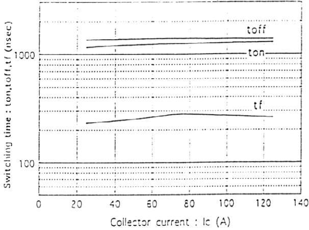
Switching time vs. Collector current Ede=300V, Vcc=15V, Tj=25°C
