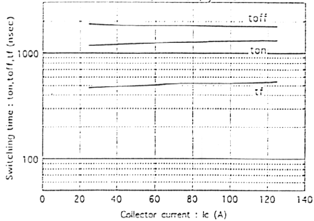
Switching time vs. Collector current Ede=300V, Vcc=15V, Tj=125°C
