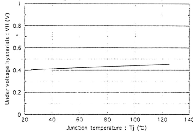
Under voltage hysteresis vs. Junction temperature
