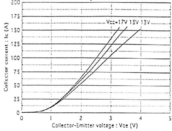
Collector current vs. Collector-Emitter voltage Tj=125°C
