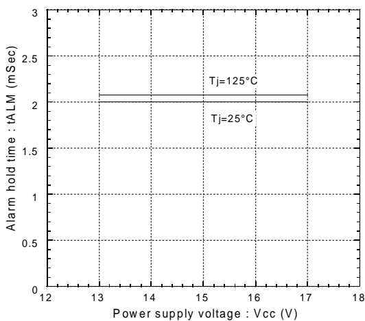
Alarm hold time vs. Power supply voltage
