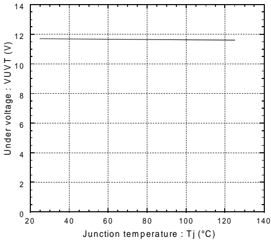
Under voltage vs. Junction temperature
