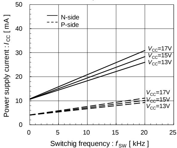
Power supply current vs. switching frequency (typ.) T_{vj} = 25^{\circ}\text{C}
