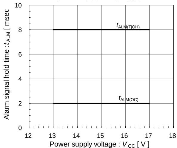
Alarm signal hold time vs. power supply voltage (typ.)
