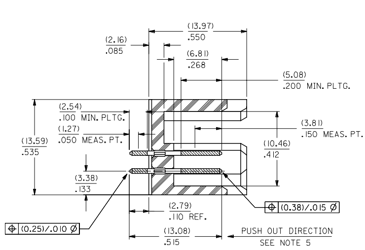
SECTION W-W
