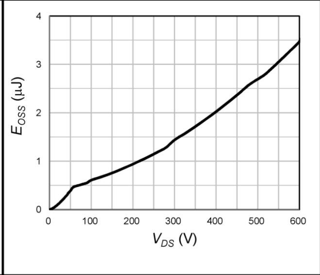
Fig.12 Output Capacitance Stored Energy
