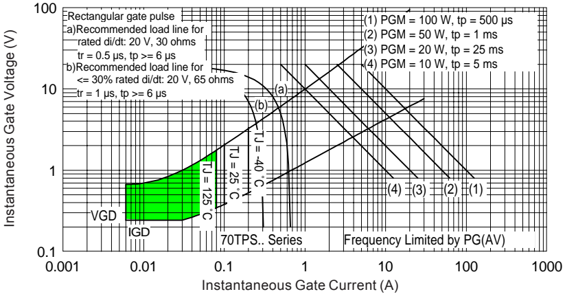
Fig. 8 - Gate Characteristics
