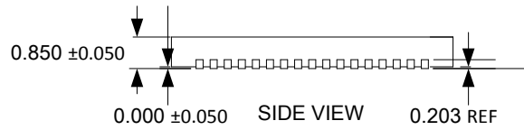
Figure 46: QFN-68 Package Outline, Top and Side View
