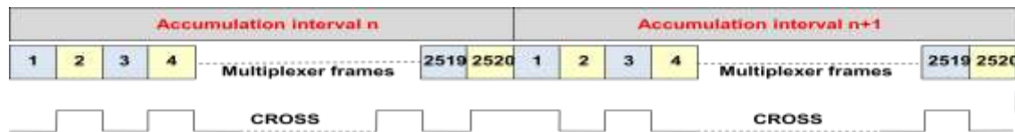
Figure 7: CROSS Signal with CHOP\_E = 00
