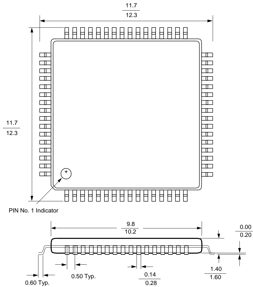
Figure 37: 64-pin LQFP Package Outline
