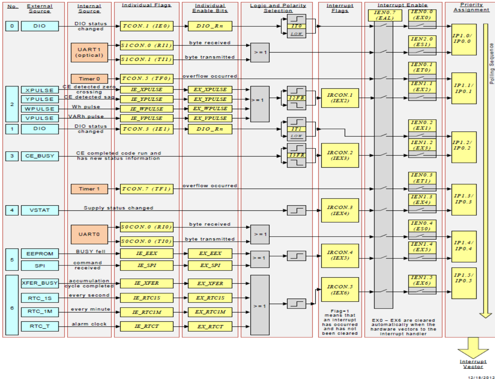
Figure 12: Interrupt Structure
