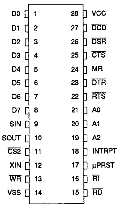
SSI 73M2550 UART 28-Pin DIP
