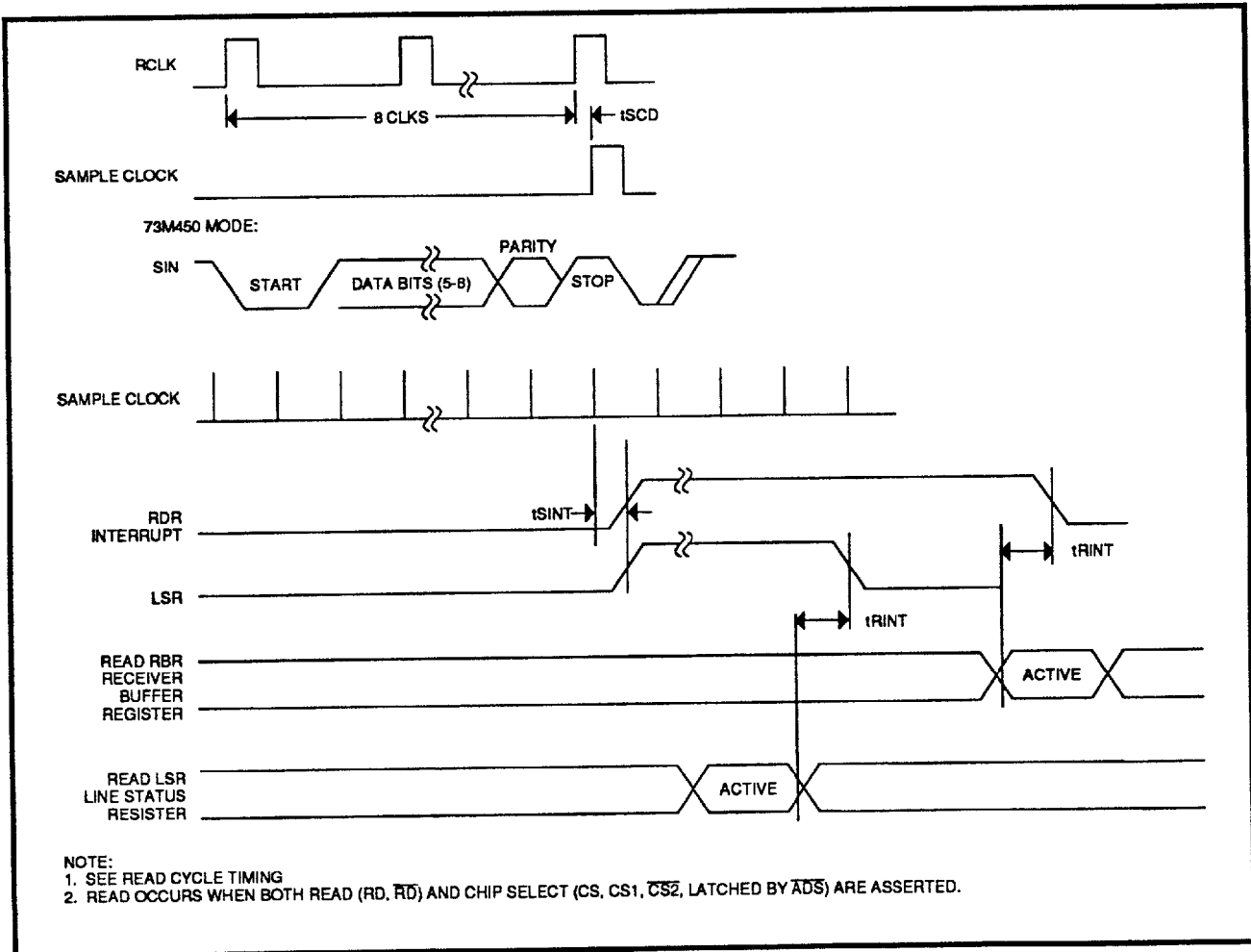
FIGURE 11: Receiver Timing
