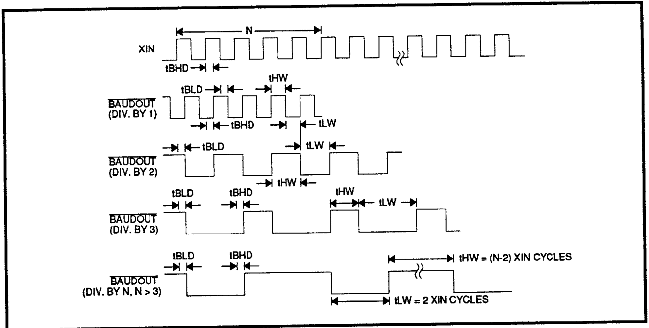
FIGURE 10: BAUDOUT Timing
