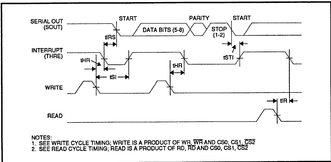
FIGURE 6: Transmitter Timing
