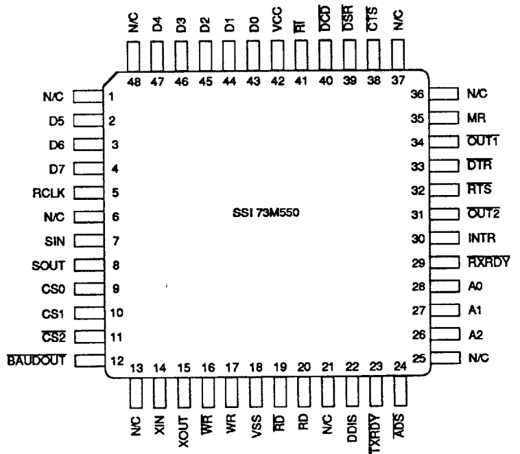
SSI 73M550 48-Lead TQFP
