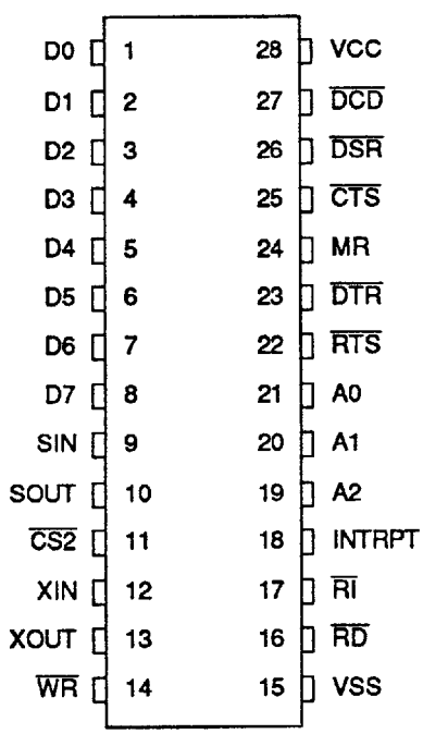
SSI 73M1550 UART 28-Pin DIP
