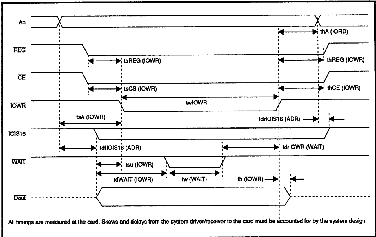
FIGURE 16: I/O Output Timing Specification (WRITE)
