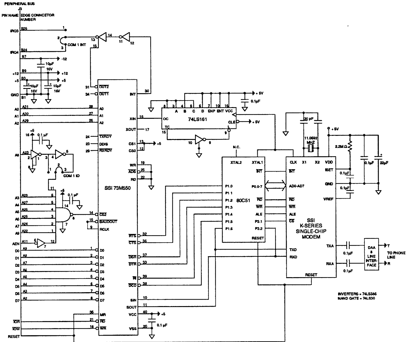
FIGURE 18: Typical Application Showing Modem Interface to Peripheral-Bus via SSI 73M550 UART
