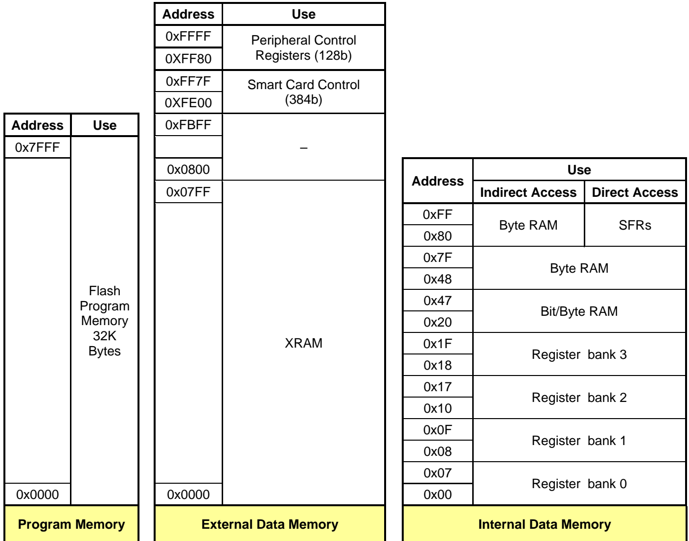
Figure 2: Memory Map
