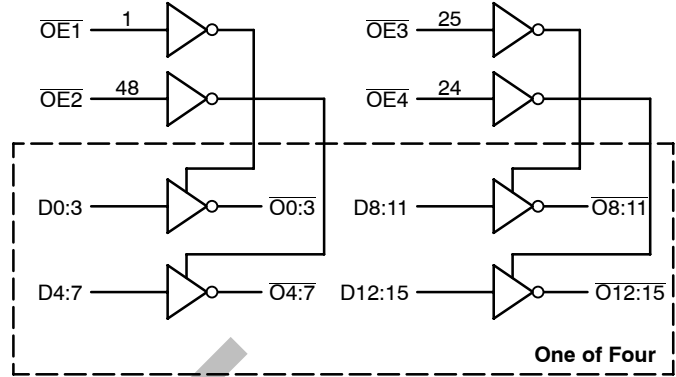
Figure 2. Logic Diagram
