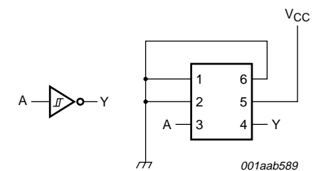
Fig 10. Inverter
