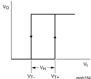
Fig 9. Transfer characteristic
