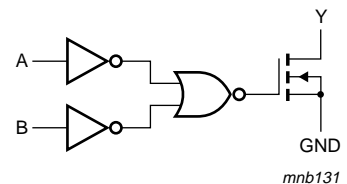
Fig 3. Logic diagram (one gate)
