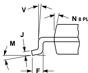
DETAIL E
