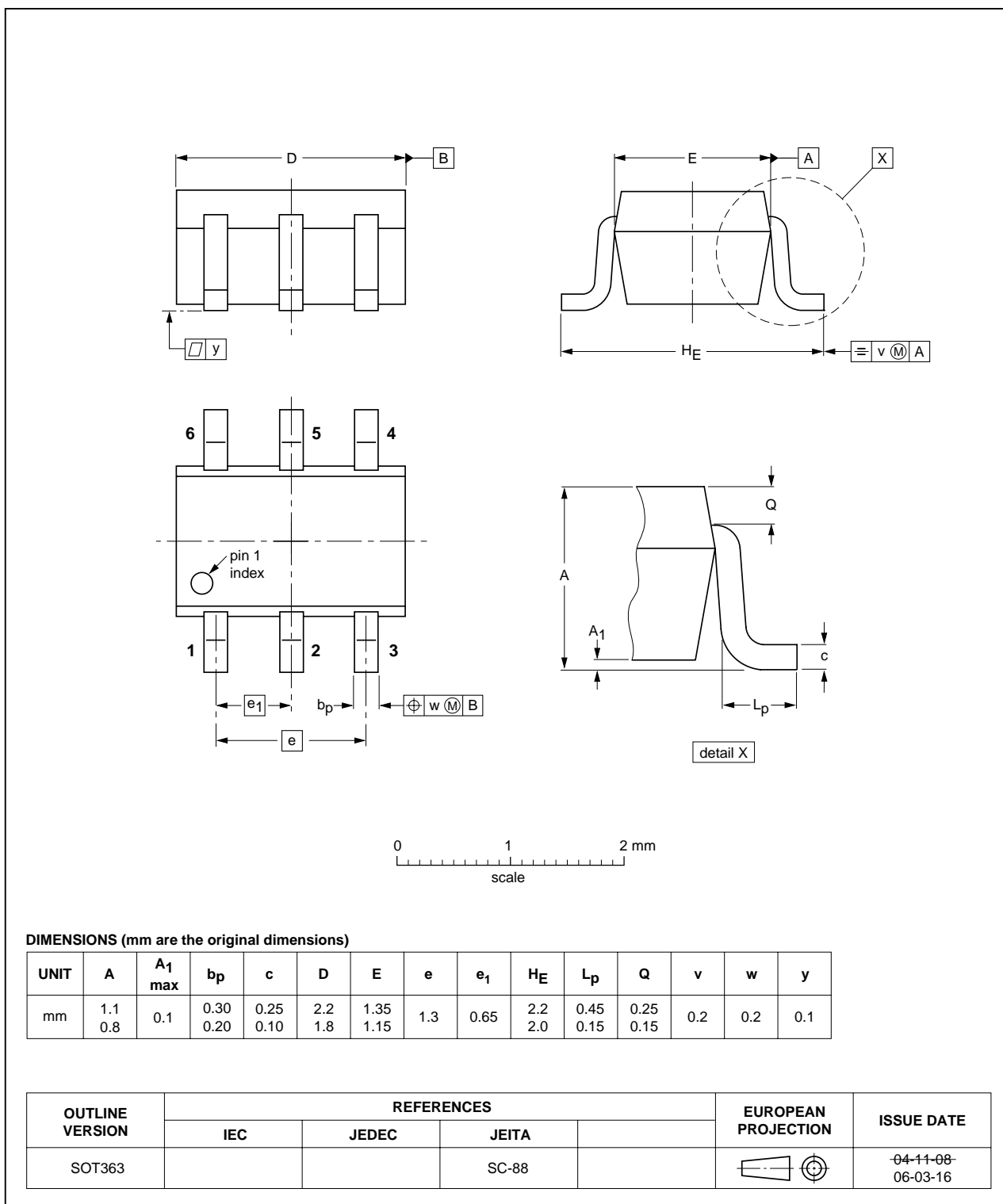
Fig 13. Package outline SOT363 (SC-88)
