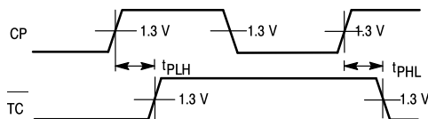
Figure 3. Clock to Terminal Delays
