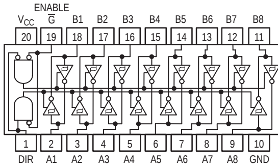
SN74LS640 SN74LS642
