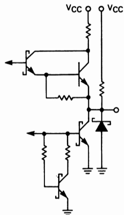
FIGURE 24 — TYPICAL INPUT
