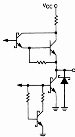
FIGURE 25 — TYPICAL OUTPUT
