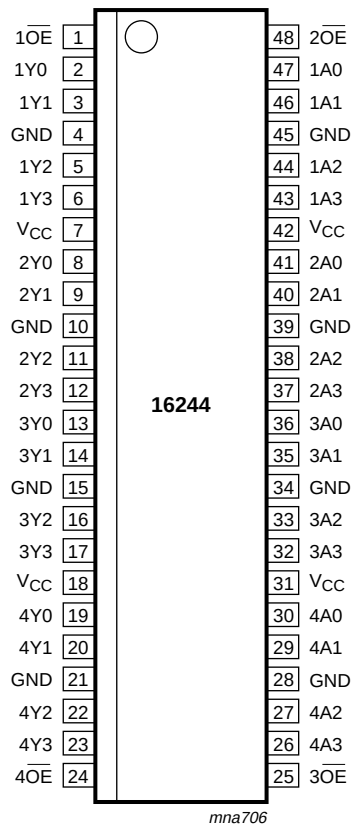
Fig.1 Pin configuration SSOP48 and TSSOP48.
