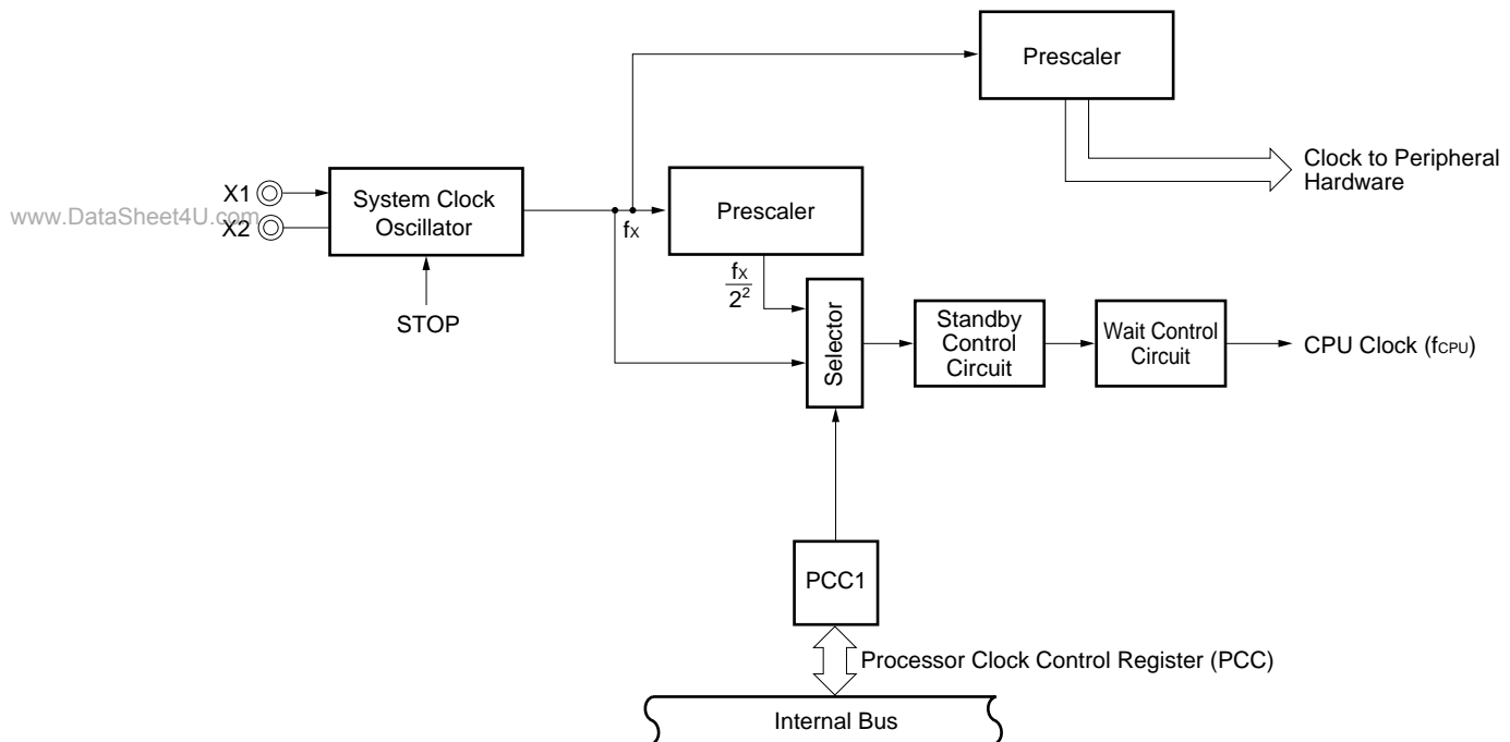
Figure 5-1. Block Diagram of Clock Generation Circuit
