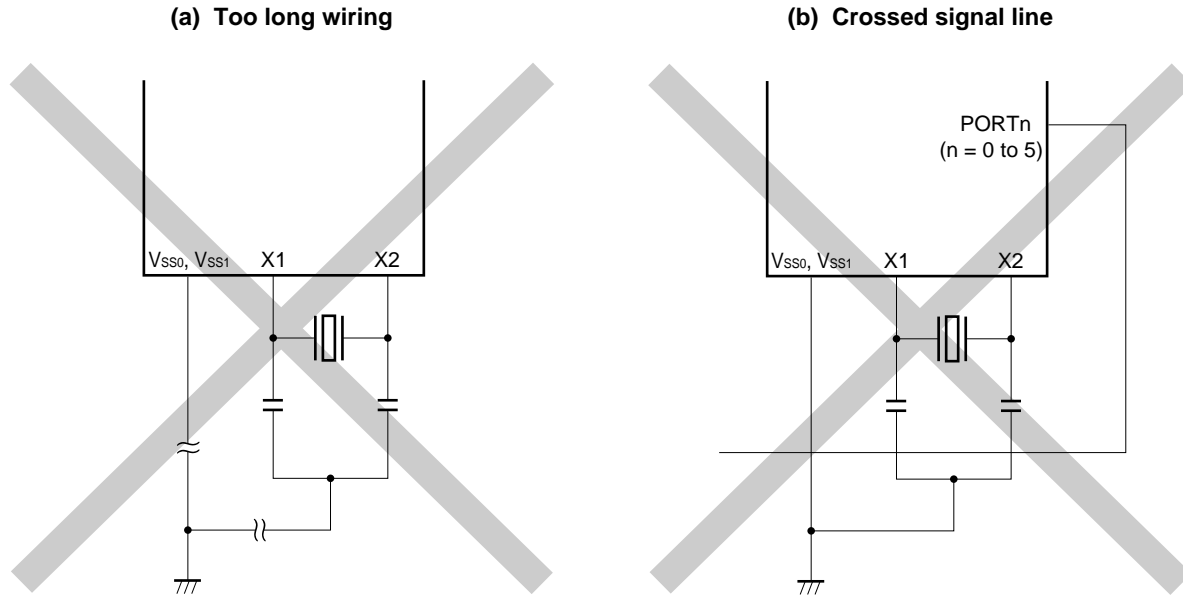
Figure 5-4. Incorrect Examples of Resonator Connection (1/2)
