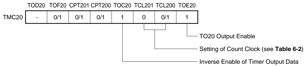
Figure 6-6. Settings of 16-Bit Timer Mode Control Register 20 at Timer Output Operation
