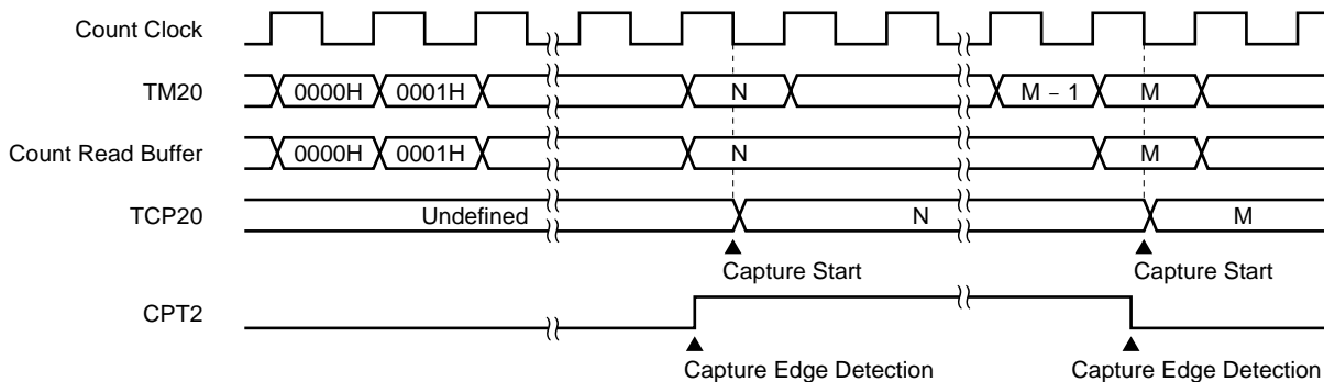
www.DataSheet4U.com Figure 6-9. Capture Operation Timing (Both Edges of CPT2 Pin are Specified)
