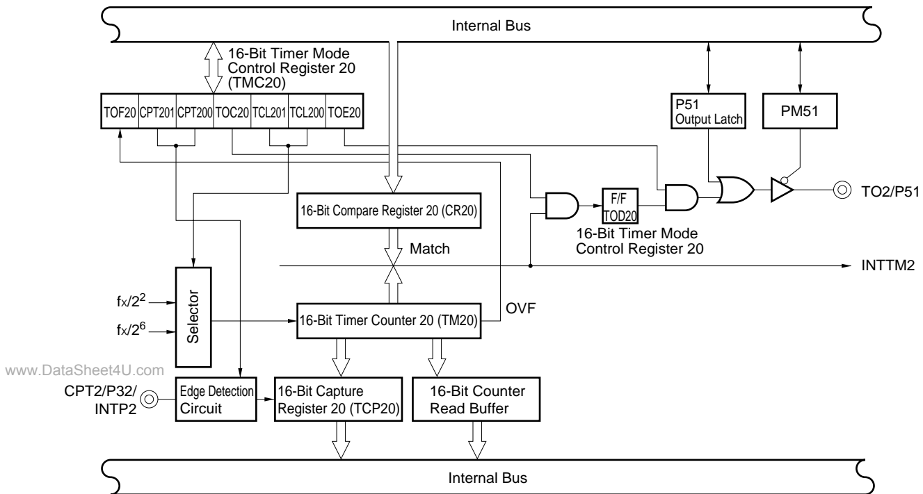
Figure 6-1. Block Diagram of 16-Bit Timer 20
