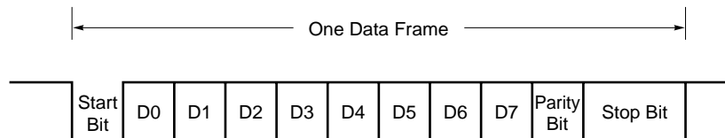
Figure 9-7. Asynchronous Serial Interface Transmit/Receive Data Format
