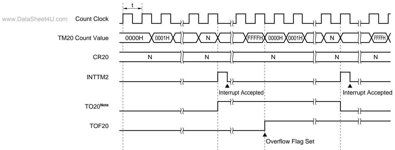
Figure 6-7. Timer Output Timing
