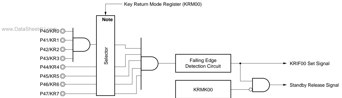
Figure 10-7. Falling Edge Detection Circuit
