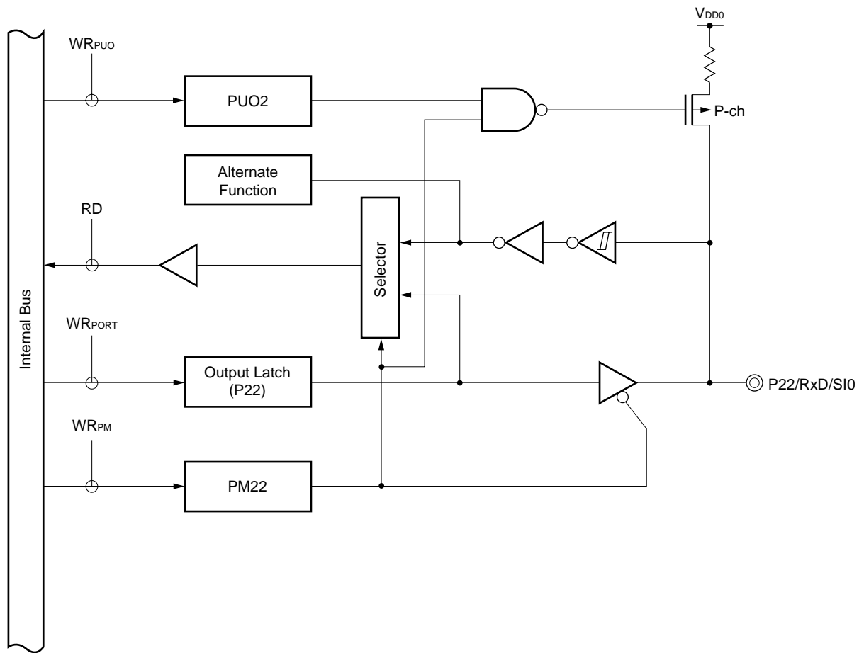
Figure 4-6. Block Diagram of P2
