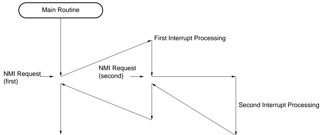
Figure 10-10. Accepting Non-Maskable Interrupt Request
