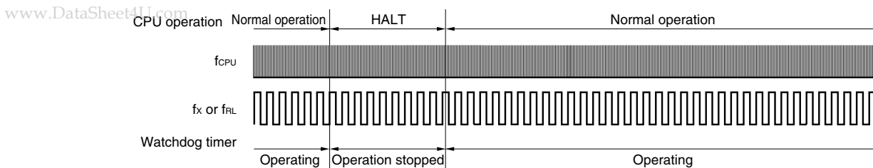
Figure 8-8. Operation in HALT Mode
