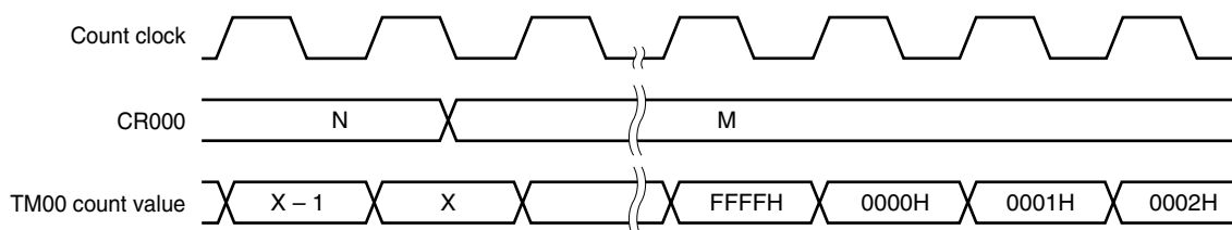
Figure 6-14. Timing After Change of Compare Register During Timer Count Operation ( N \rightarrow M : N > M )
