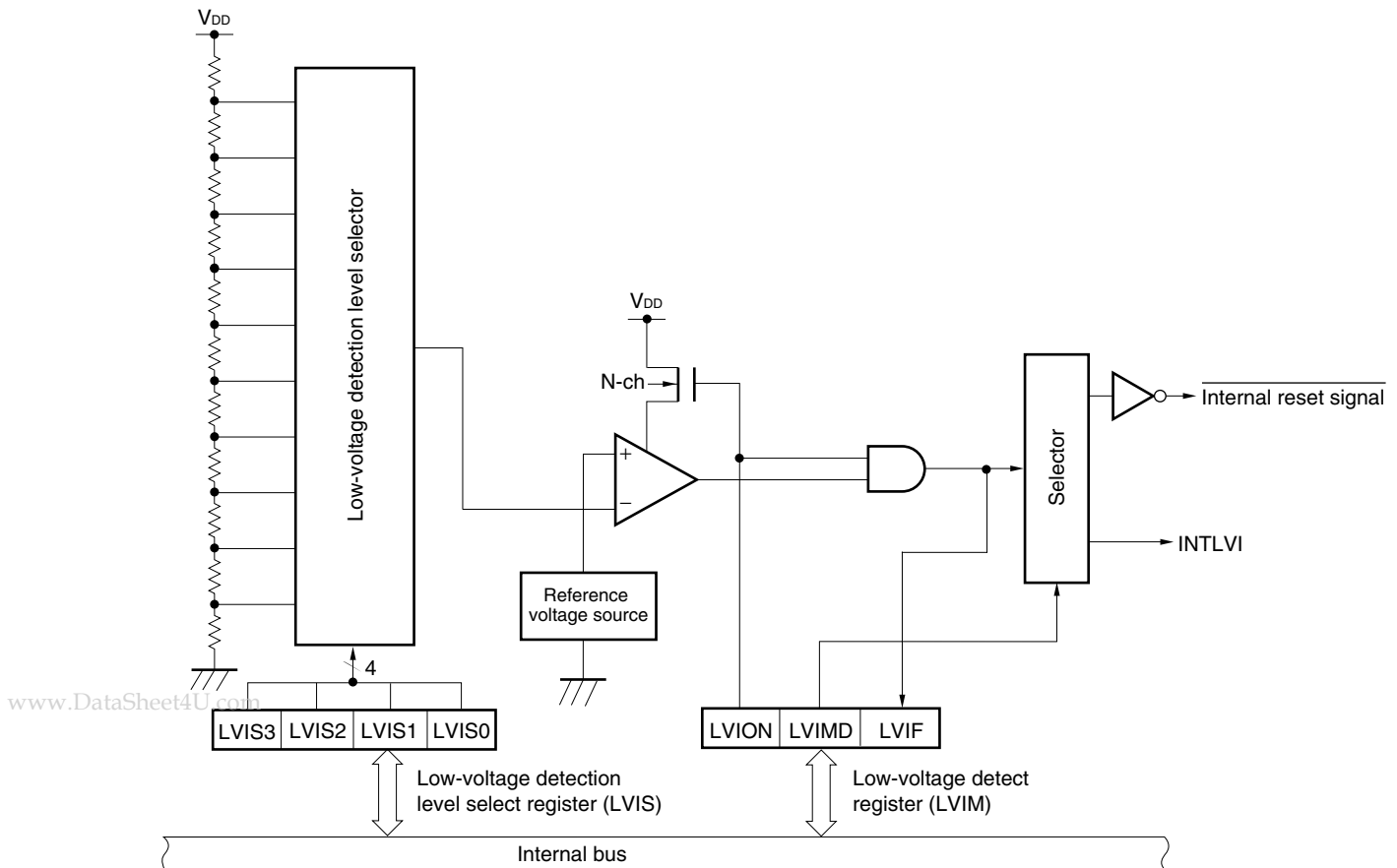
Figure 14-1. Block Diagram of Low-Voltage Detector
