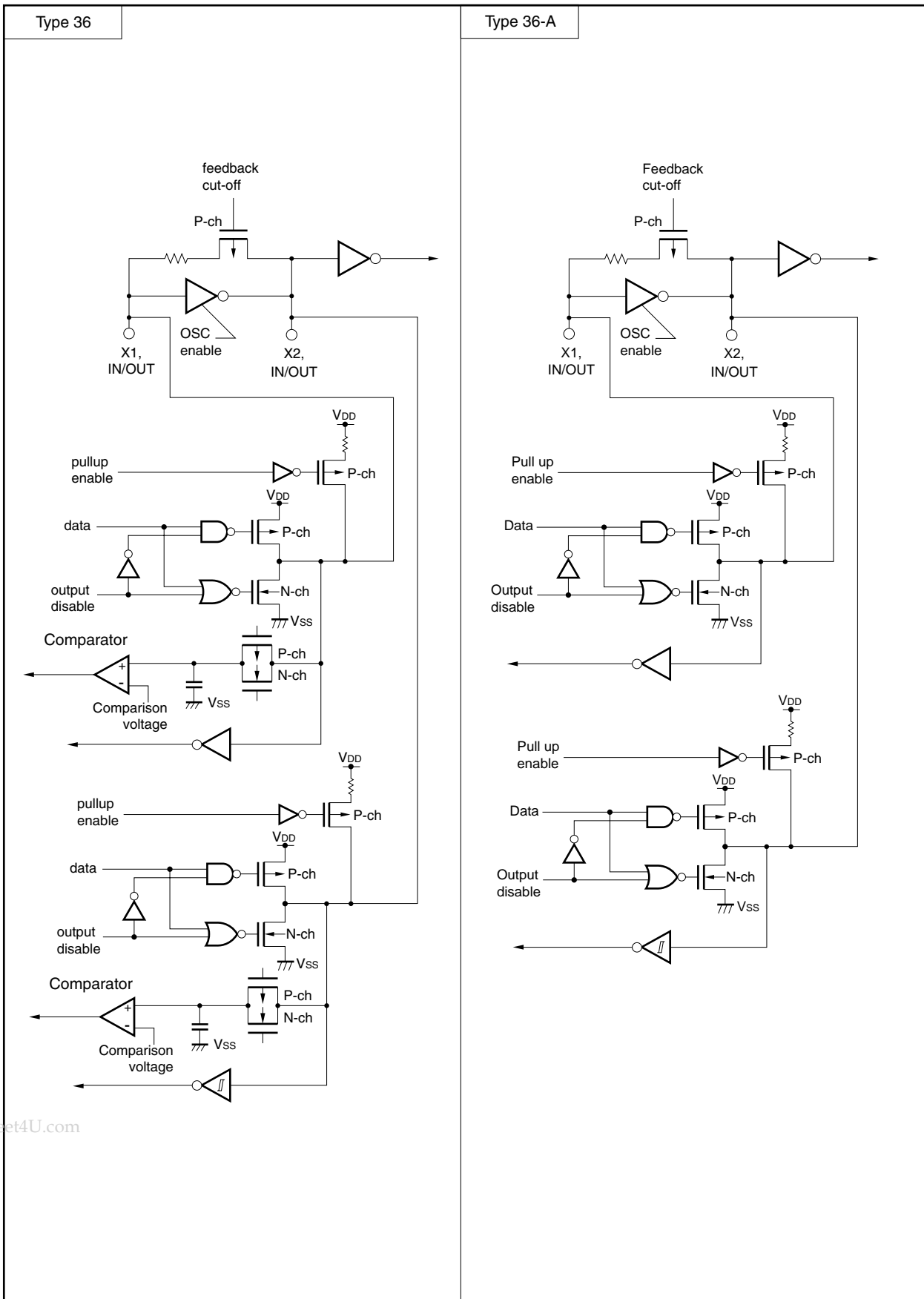
Figure 2-1. Pin I/O Circuits (2/2)
